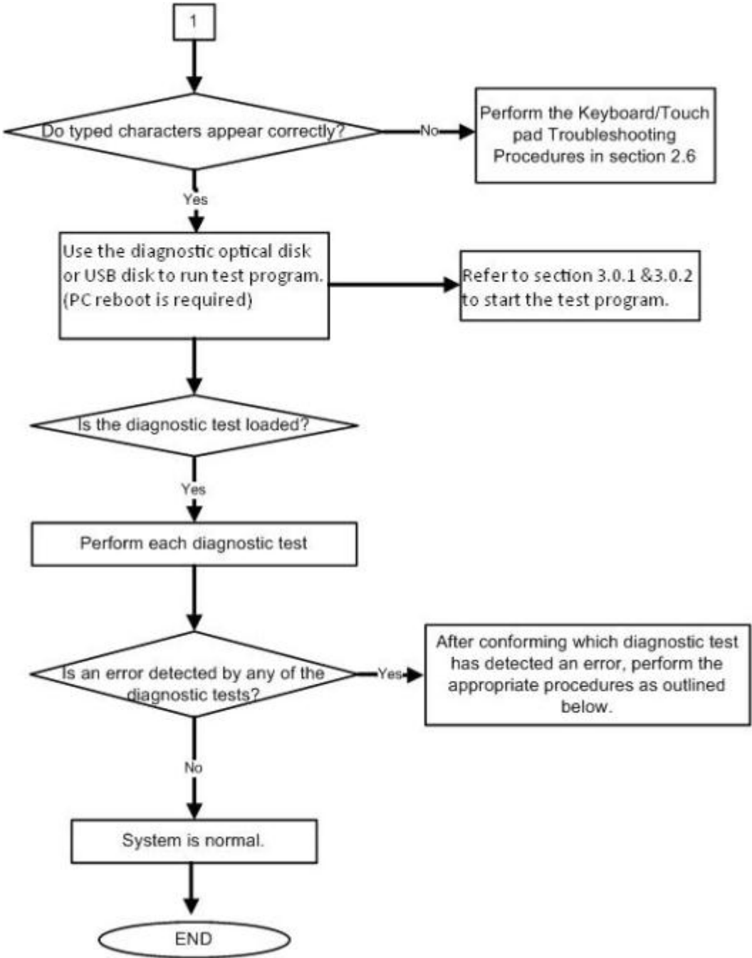
Figure 2-1 Troubleshooting flowchart (2/2)
